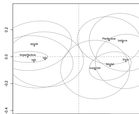
Figure 13 Binary correspondence analysis joint plot, function anacor , package {anacor}
