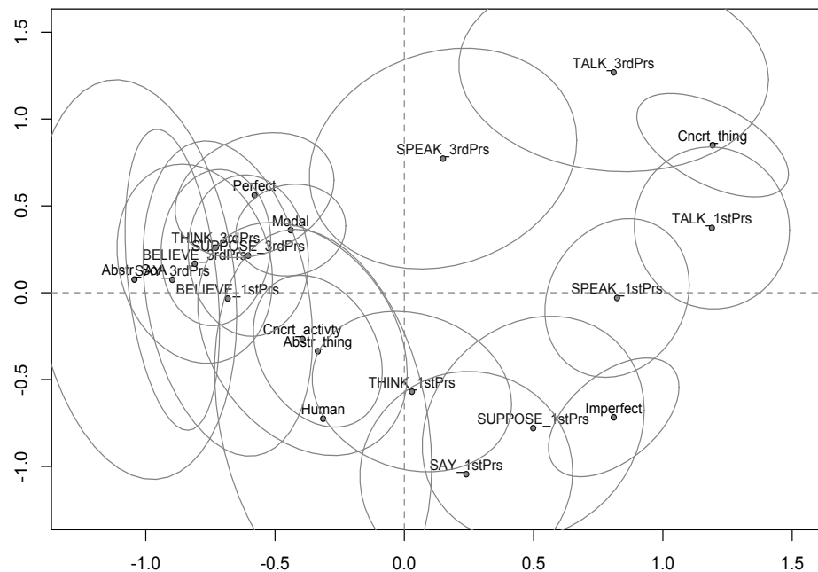
Figure 9. Binary Correspondence Analysis, scaling “standard” vs. “standard” function res , package {anacor} , plot type “ jointplot ”
