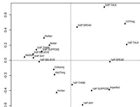
Figure 15. Multiple correspondence analysis biplot, function mjca , package {ca}
