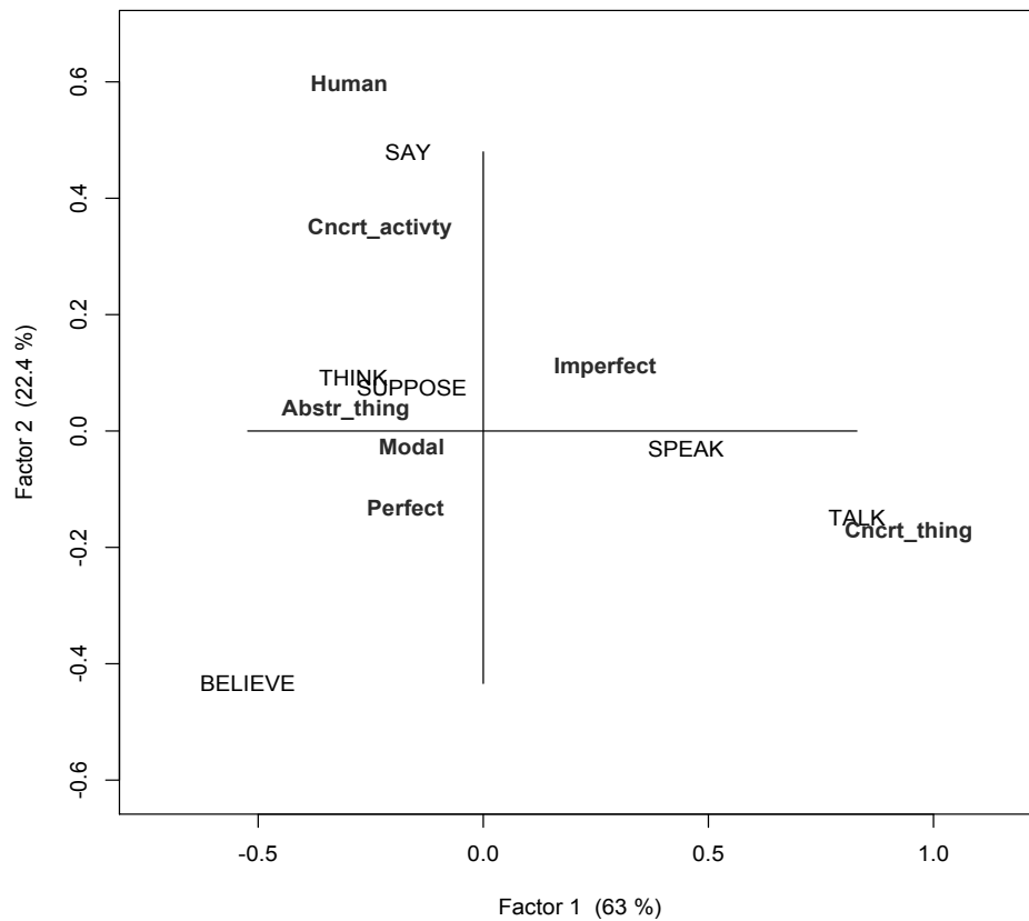
Figure 4. Binary correspondence analysis, from Table 3, function corres.fnc , package {languageR}
