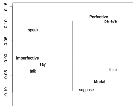
Figure 11 Binary correspondence-analysis biplot, function corres.fnc , package {languageR}
