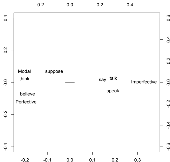
Figure 1. Binary correspondence analysis, function corresp , package {MASS}
