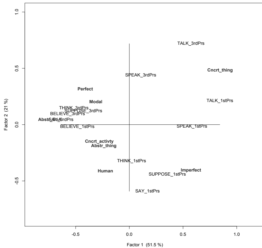
Figure 5. Binary correspondence analysis, from Table 4, function corres.fnc , package {languageR}
