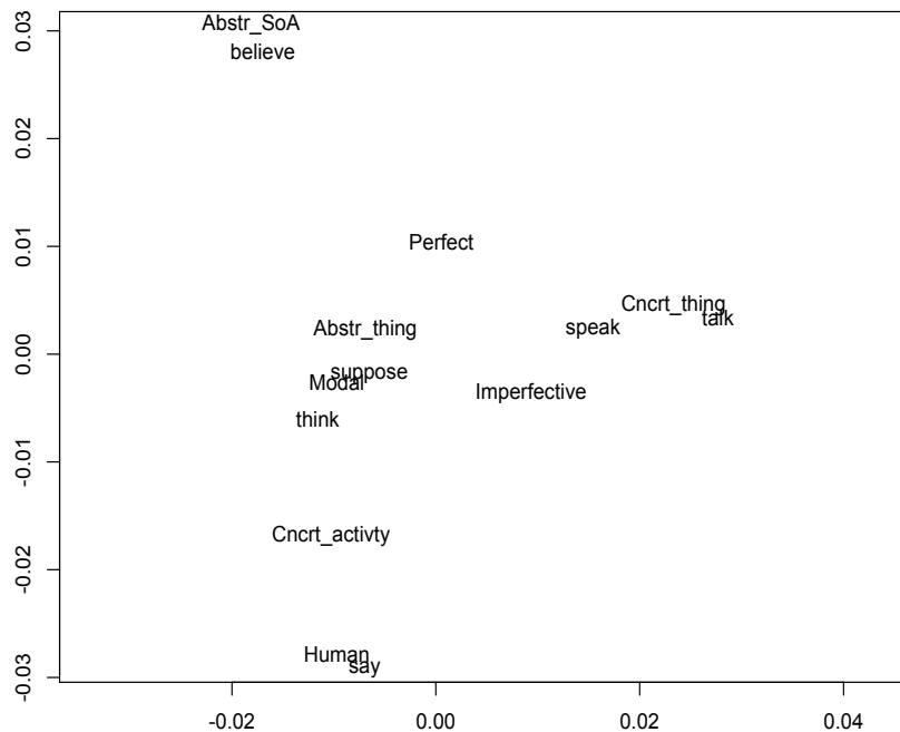
Figure 2. Multiple correspondence analysis, function mca , package {MASS}
