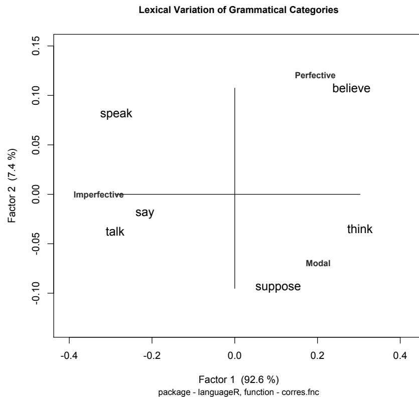
Figure 3. Binary correspondence analysis, function corres.fnc , package {languageR}
