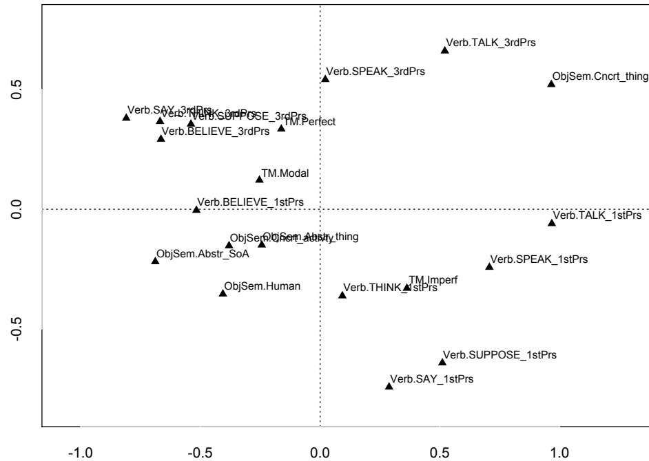
Figure 7. Joint multiple correspondence analysis function mjca , package {ca} , method= JCA
