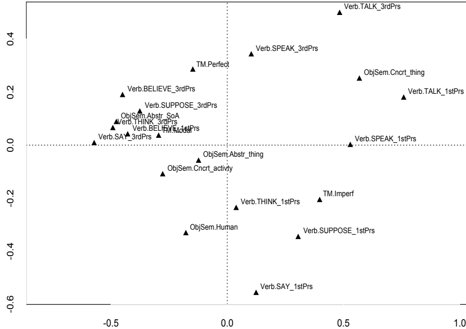
Figure 8. Burt matrix multiple correspondence analysis (with adjusted inertias) function mjcA , package {ca} , method= adjusted
