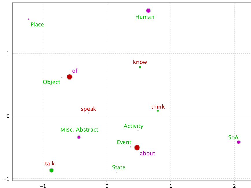
Figure 2. Association of complement, predicate and object semantics Multiple correspondence analysis (Burt matrix method) 10
